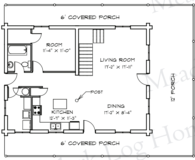
MAIN FLOOR 1064 sq. ft.
