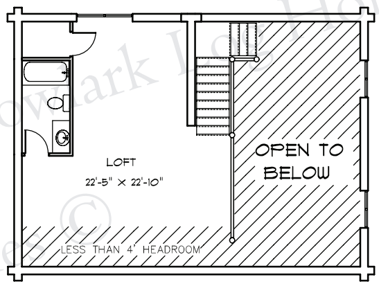
LOFT 505 sq. ft.
