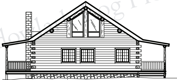
BACK ELEVATION
